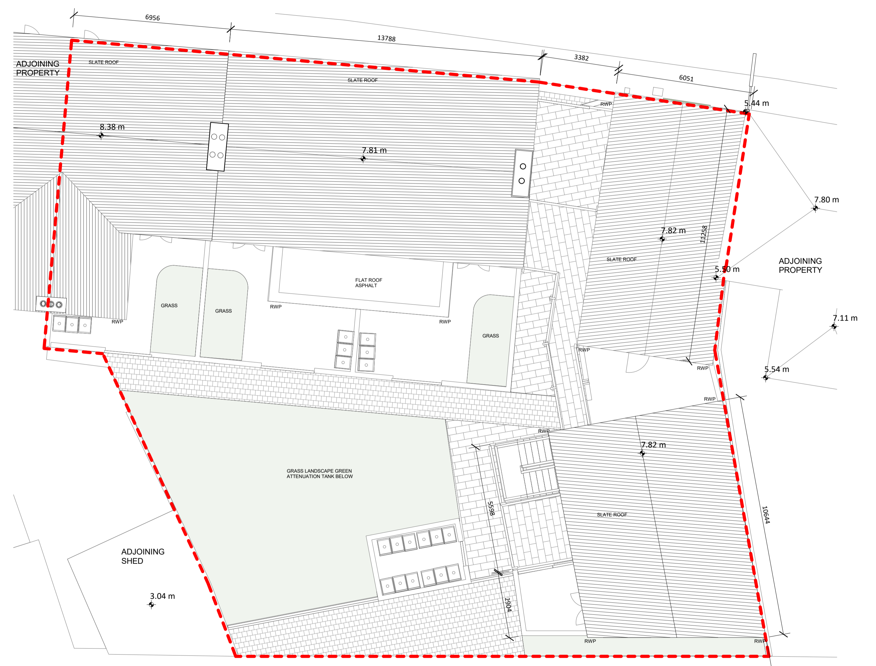
GA ROOF PLAN Scale 1:100
