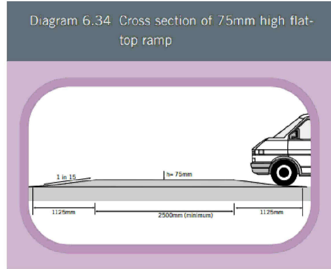
TYPICAL CROSS SECTION DETAIL OF 75MM HIGH PEDESTRIAN RAMP
